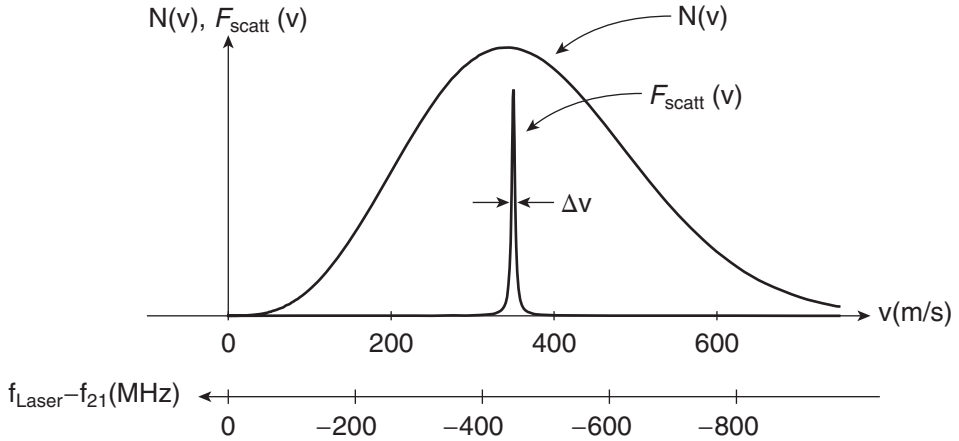
FIGURE 16.8 Maxwellian velocity distribution of a rubidium atomic beam at 400^\circ\text{C} and the magnitude of the scattering force for a laser tuned 450 MHz below resonance. The narrow width of the scattering force arises from the spontaneous emission line width of the resonance transition.
