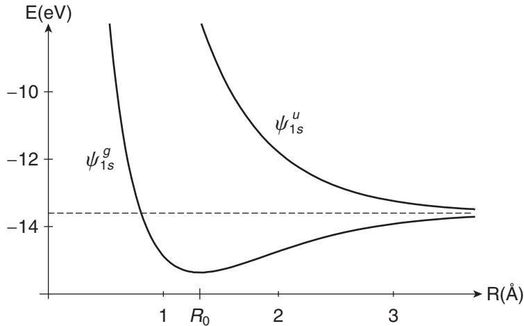
FIGURE 13.14 Energies of the bonding and antibonding orbitals of the hydrogen molecular ion, as a function of the internuclear separation.
