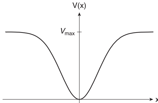
FIGURE 16.1 Generic potential energy for a particle trap in one dimension. Particles with kinetic energy less than V_{\max} are trapped in the vicinity of the origin, where the potential energy is a minimum.
