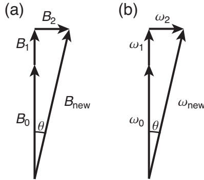
FIGURE 10.3 (a) Perturbing magnetic fields and (b) the resultant Larmor frequencies.
