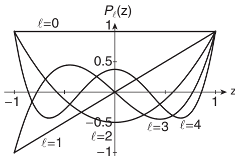
FIGURE 7.13 Legendre polynomials.
